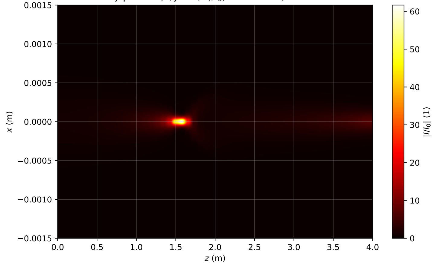
Intensity profile I(x, y = 0, z)/I_0 , P_{in}=1.6P_{cr} , artificial time
